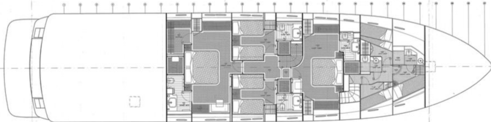
Pianta Lower Deck
