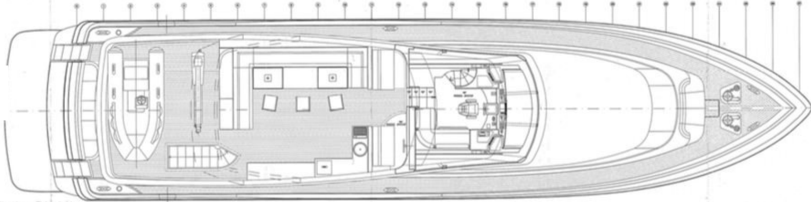
Pianta - Flying Bridge
