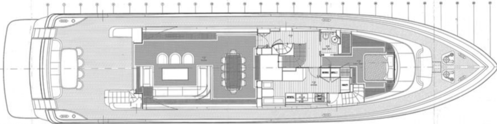
Pianta Main Deck
