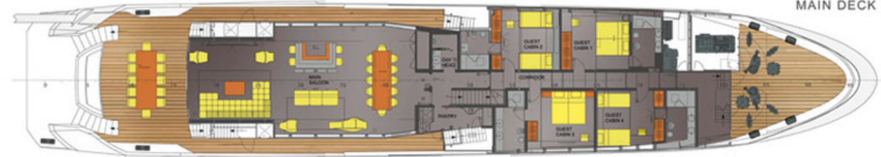
MAIN DECK
