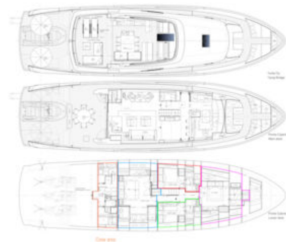
OZONE - Layout
